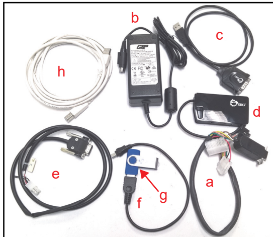
Figure 1 GEN Printer Download Kit (P/N 701-000254R)
