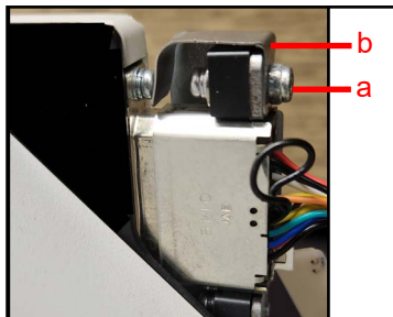
Figure 1 iVIZION® Rear Harness Connector w/ Frame Ground Plate
